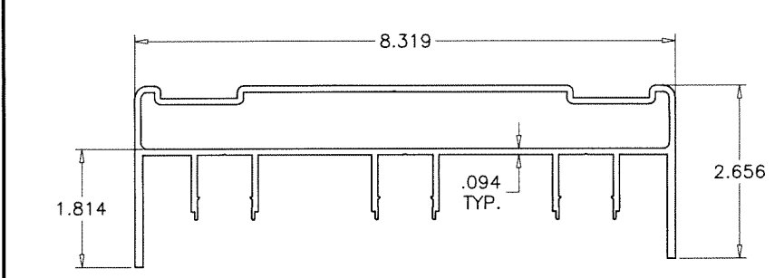
E14 FRAME HEAD AT RECEPTOR
